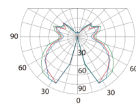
6000 - HQI - 250w
